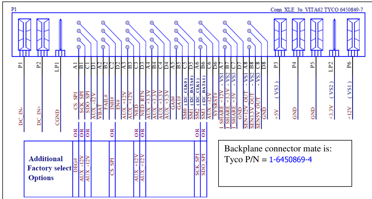
(Connector pin out – VITA 62 Compliant – Card Connector Face View)
