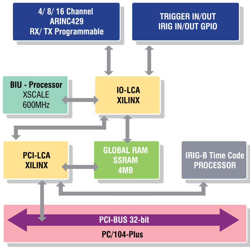
AP104-429-16 Block Diagram
