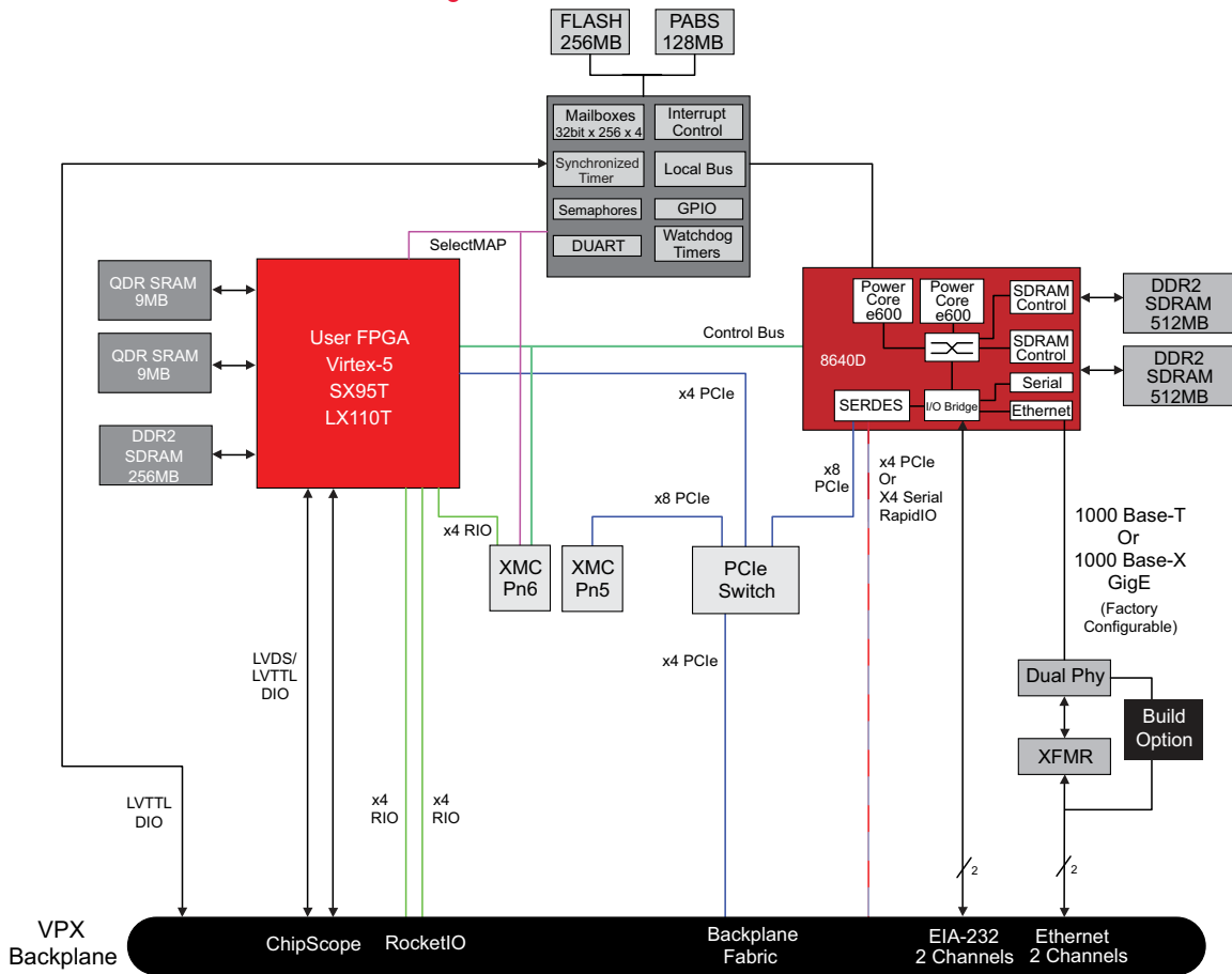
Figure 1: VPX3-450 Architecture
