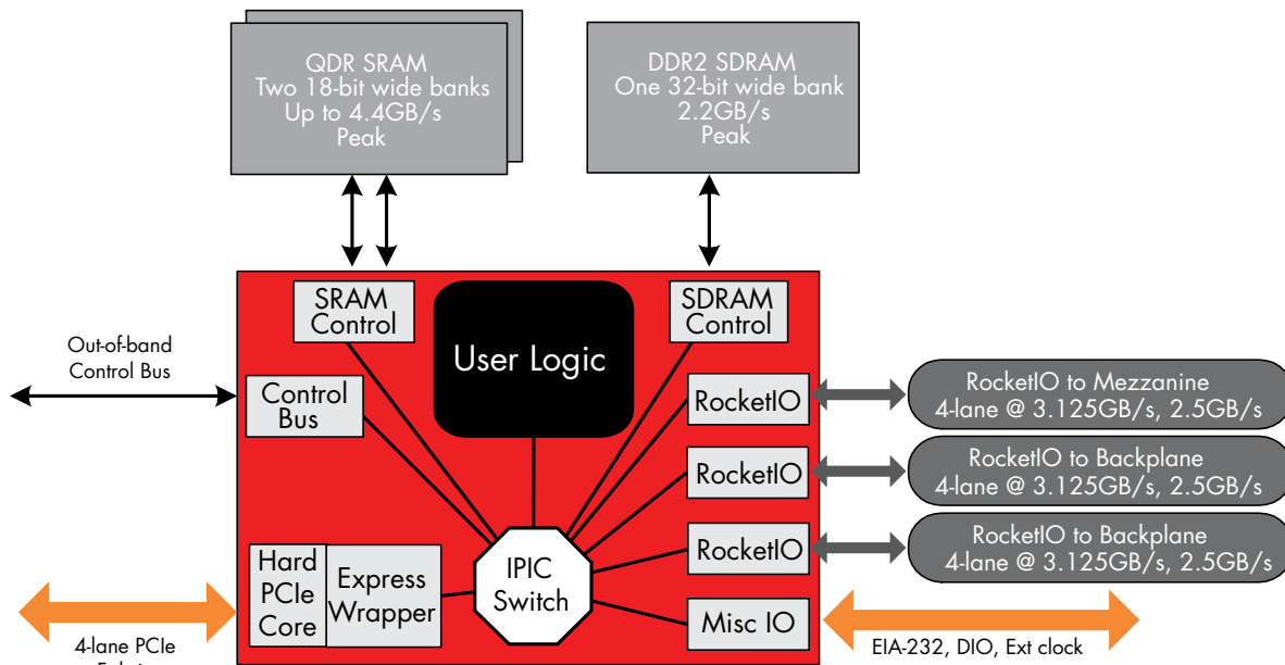
Example VPX3-450 Architecture for Xilinx Virtex-5 LX110T or SX95T
