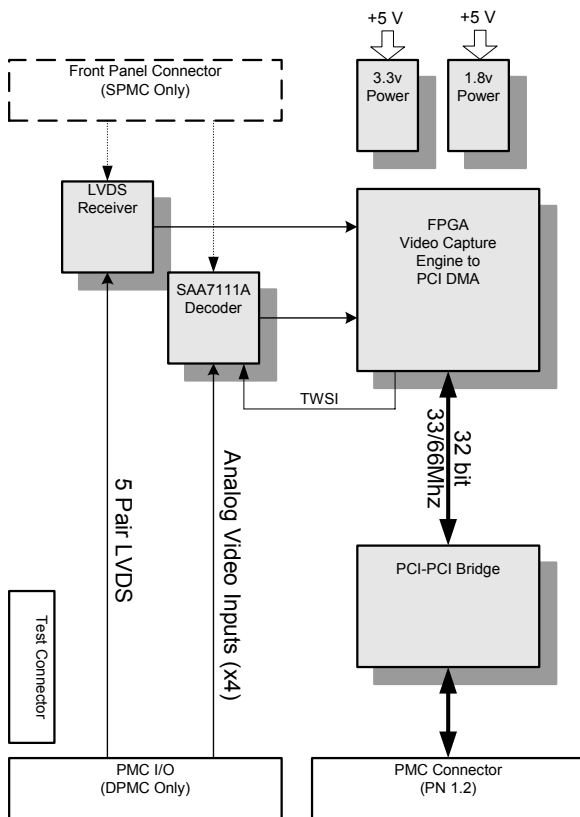
Figure 1: PMC-724 Frame Grabber Block Diagram
