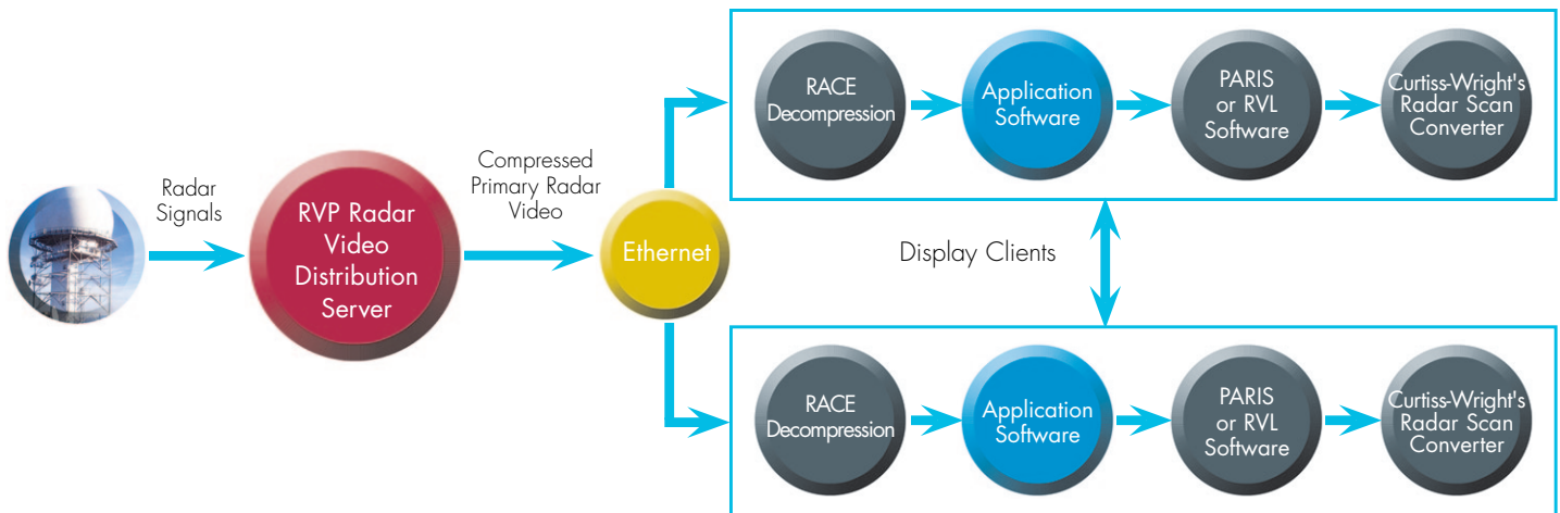
Figure 3: Structure of a Typical RVP-based Radar Video Application
