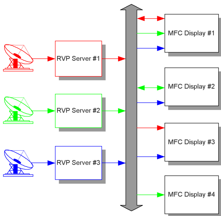
Figure 2: RVP Facilitates the Creation of Multi-Radar Multi-Console Networks
