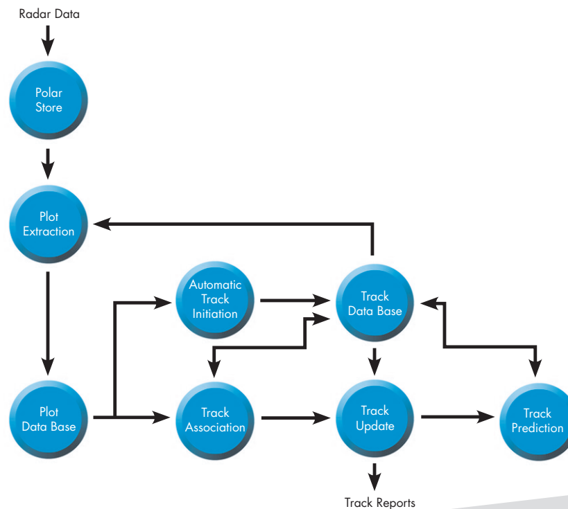
Figure 5: Data Flow Through the Plot Extraction and Target Tracking Modules
