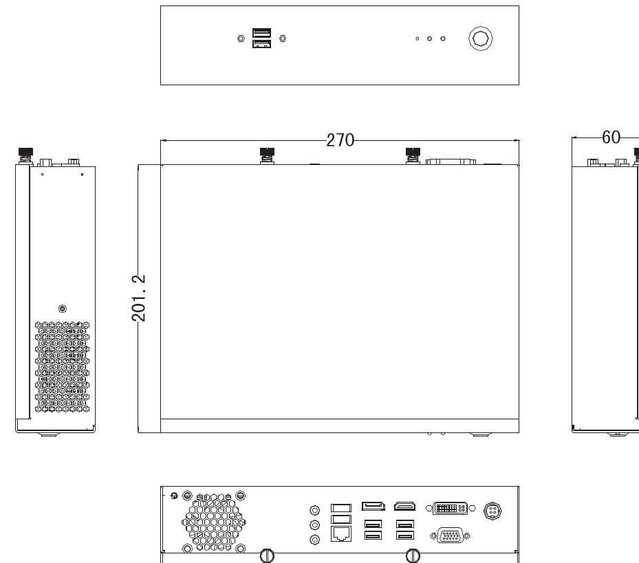
Unit: mm
