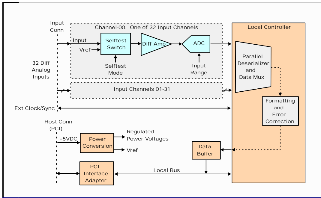
Figure 1. PMC66-16AI32SSC; Functional Organization
