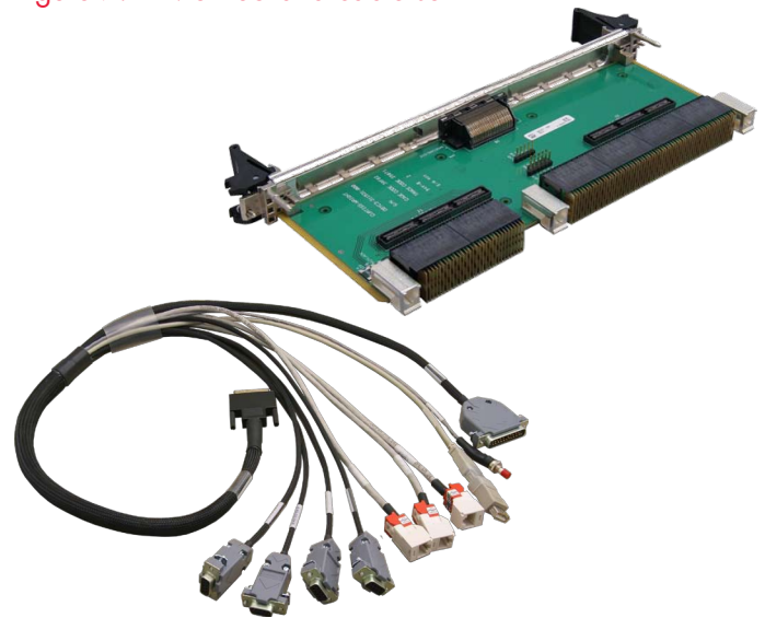
Figure 7: RTM6-185 and cable set
