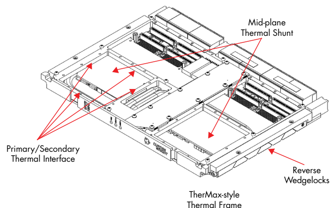
Figure 4: Representative Thermal Frame
