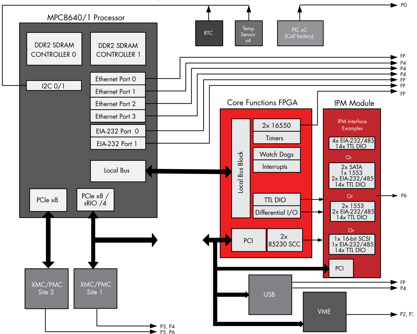
Figure 3: I/O Subsystem Diagram
