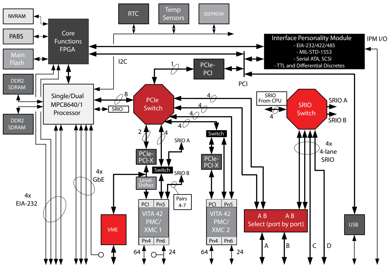
Figure 1: VPX6-185 VPX Block Diagram
